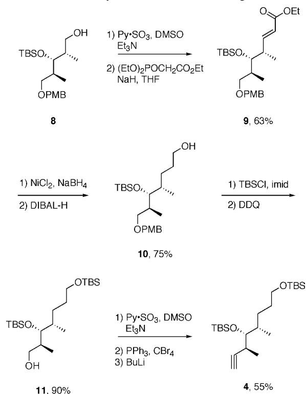
Scheme 1. Synthesis of the Middle Fragment 4
